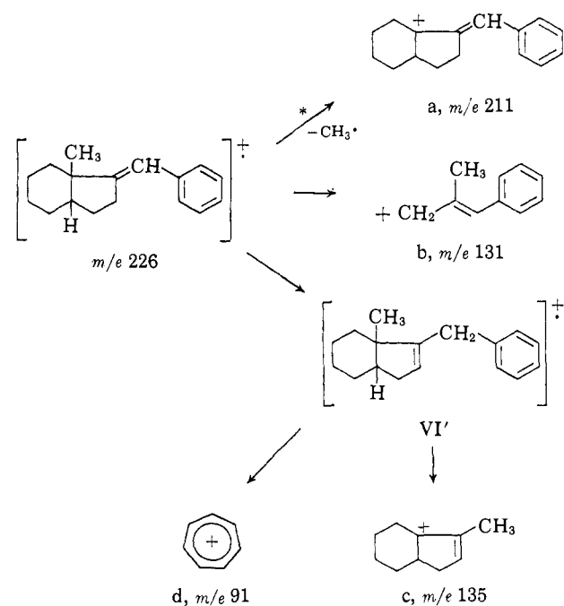
Scheme V. Major Fragmentation Pathways of cis -1-Benzylidene-8-methylhydrindan (VI) after Electron Impact
